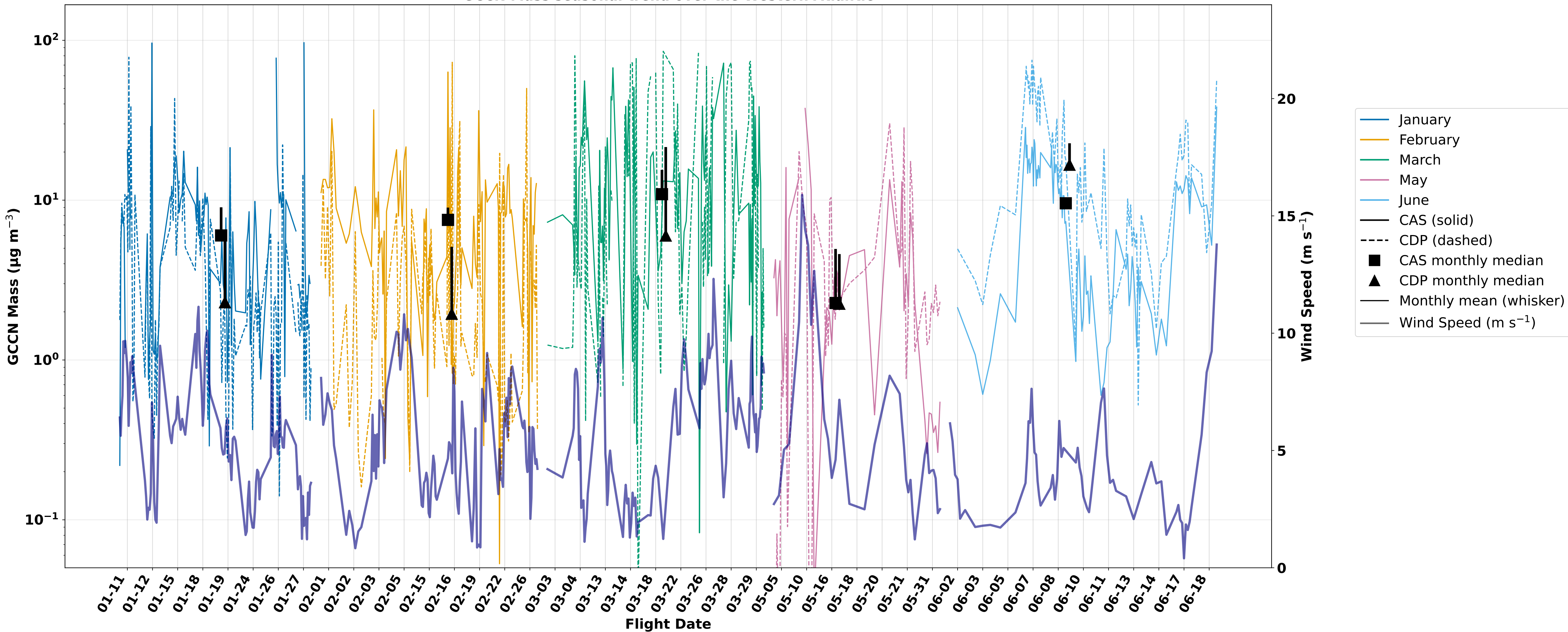
GCCN Mass seasonal trend over the Western Atlantic
